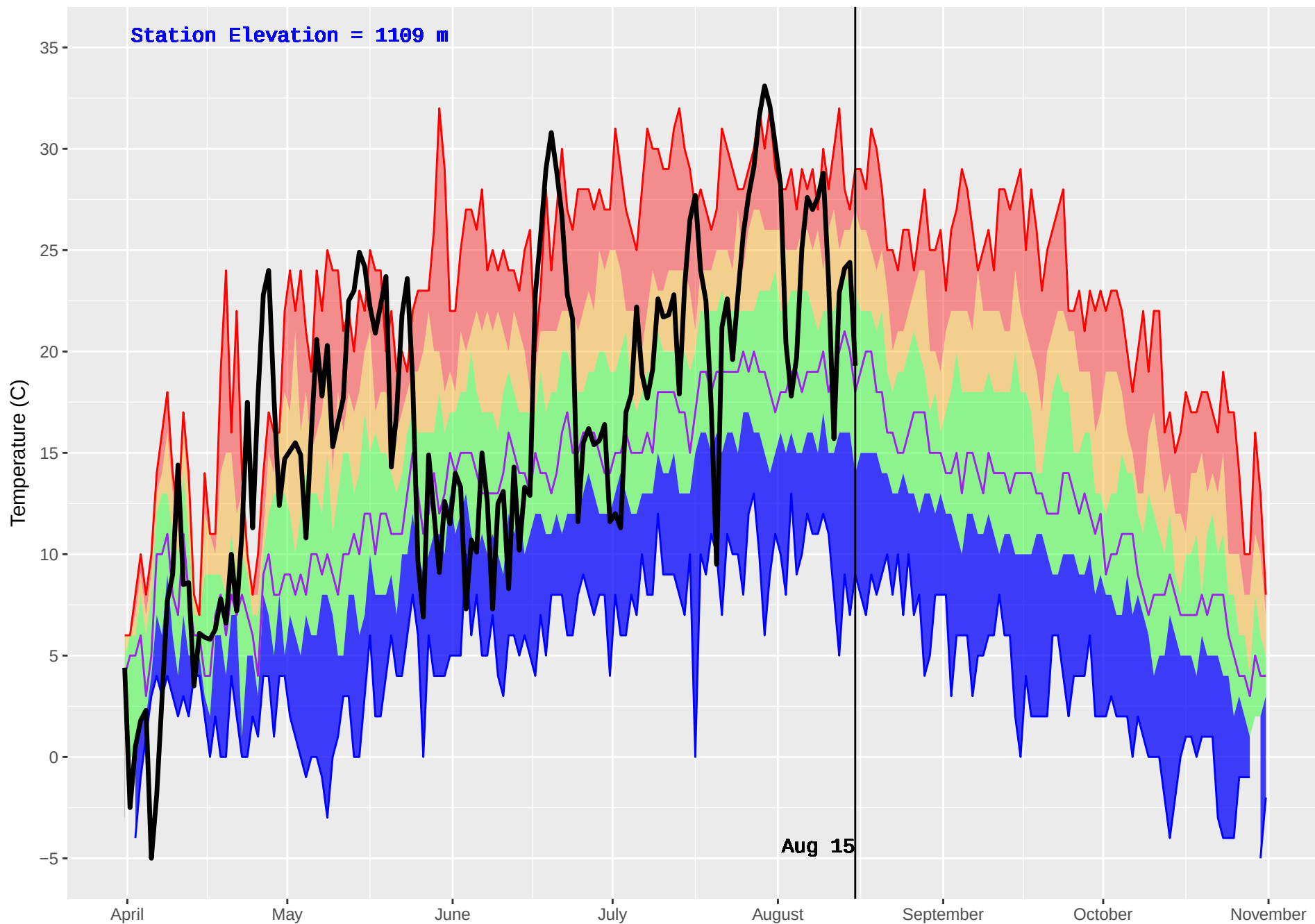
MOOSE LAKE (165) : Historical (1980–2016) and Current (2018) Daily Temperature
