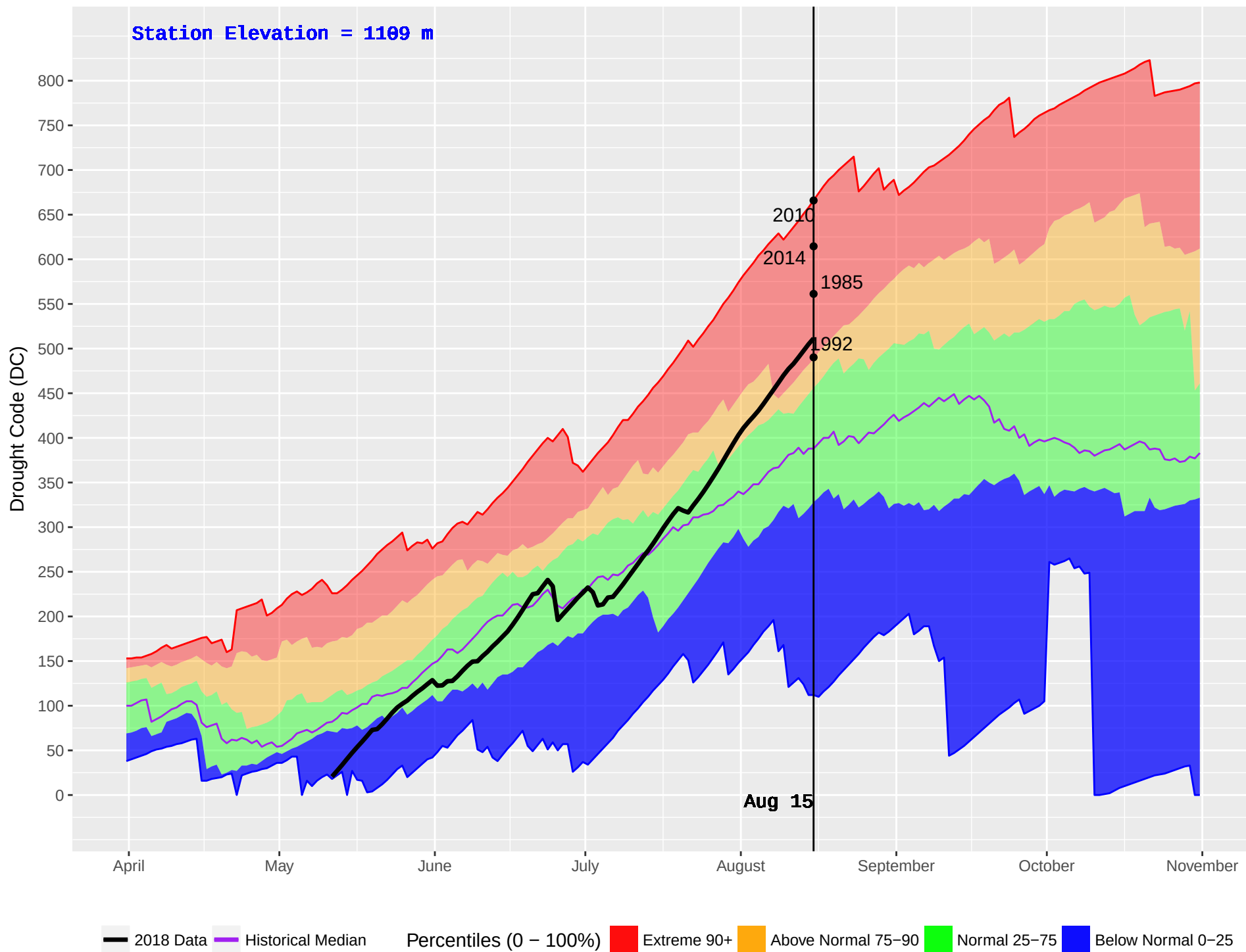
MOOSE LAKE (165) : Historical (1980–2016) and Current (2018) Daily Drought Code (DC)
